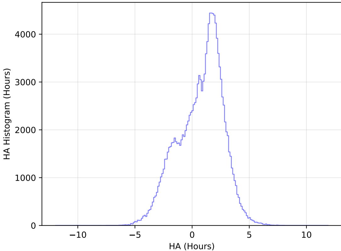
internal_u_expt45_nscale1.2v3.4_10yrs All sky u band: HA Histogram
