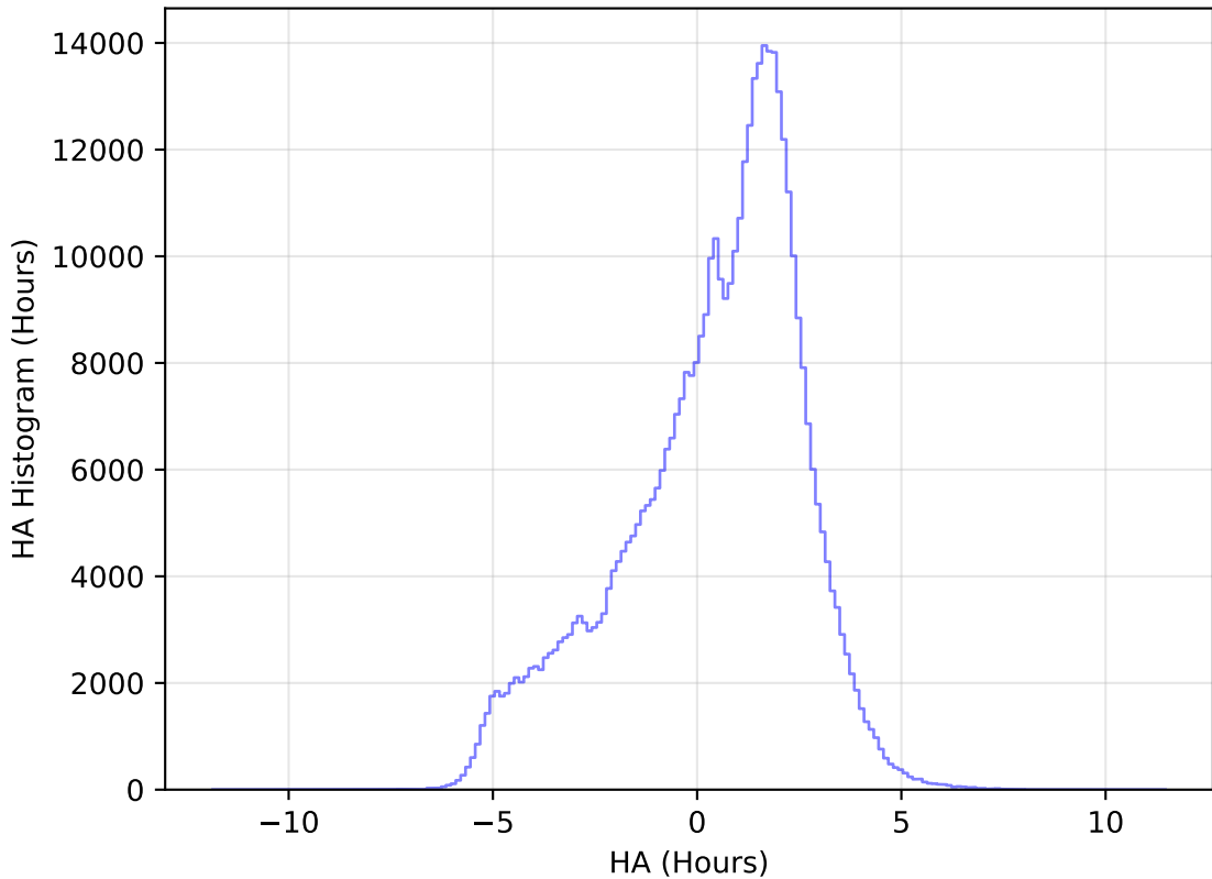
internal_u_expt45_nscale1.2v3.4_10yrs All sky r band: HA Histogram
