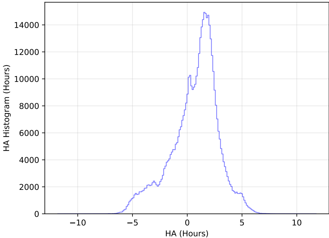
internal_u_expt45_nscale1.2v3.4_10yrs All sky i band: HA Histogram
