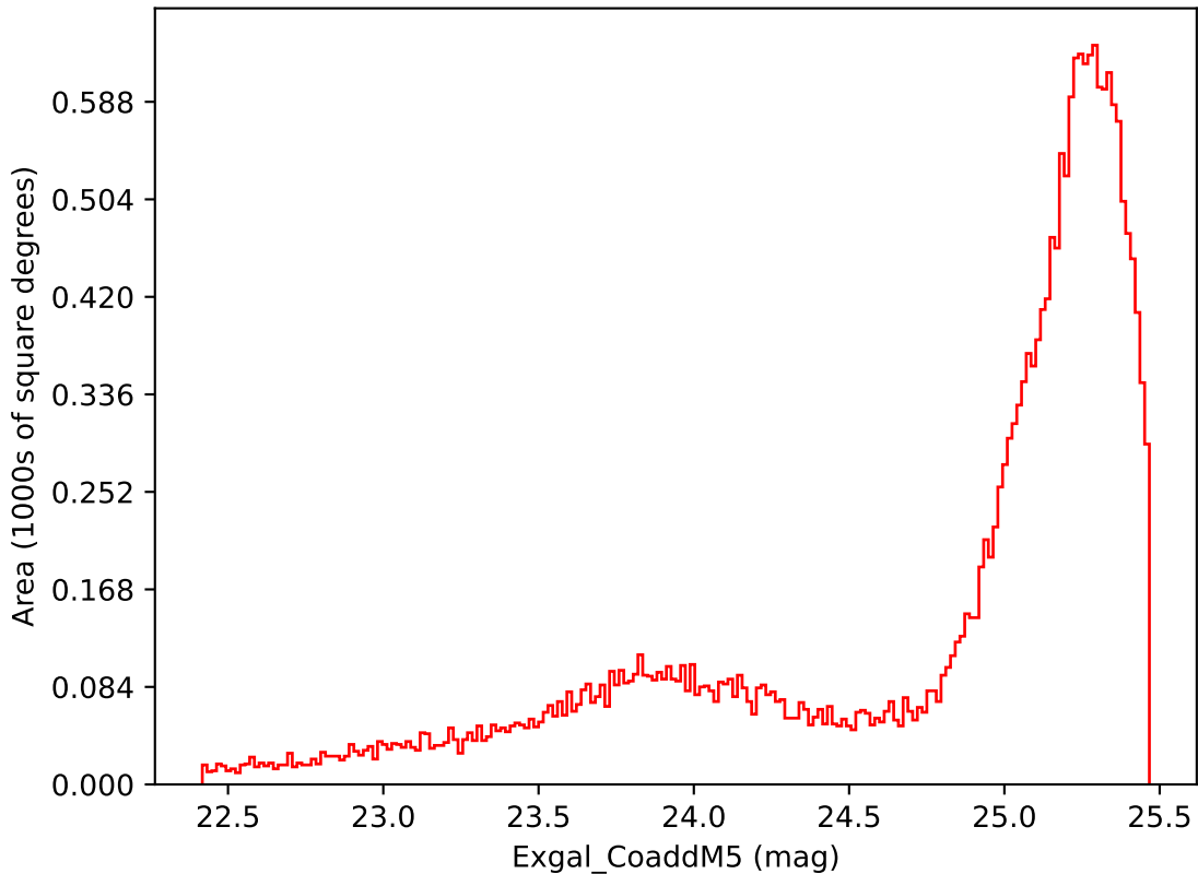
internal_u_expt45_nscale1.2v3.4_10yrs Yr 1 i band: Exgal_CoaddM5
