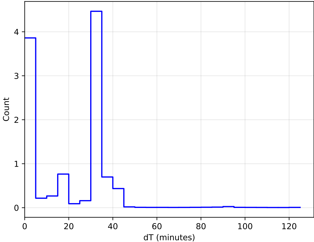
internal_u_expt45_nscale1.2v3.4_10yrs WFD: DeltaT Histogram
