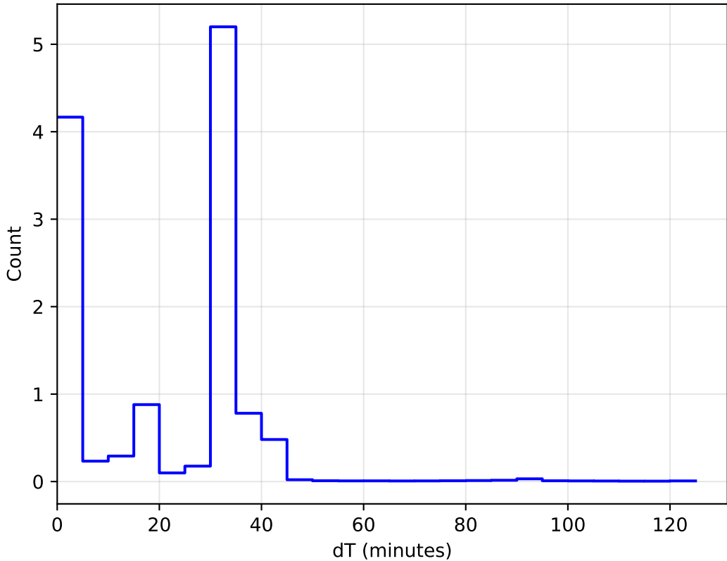
internal_u_expt45_nscale1.2v3.4_10yrs All sky: DeltaT Histogram
