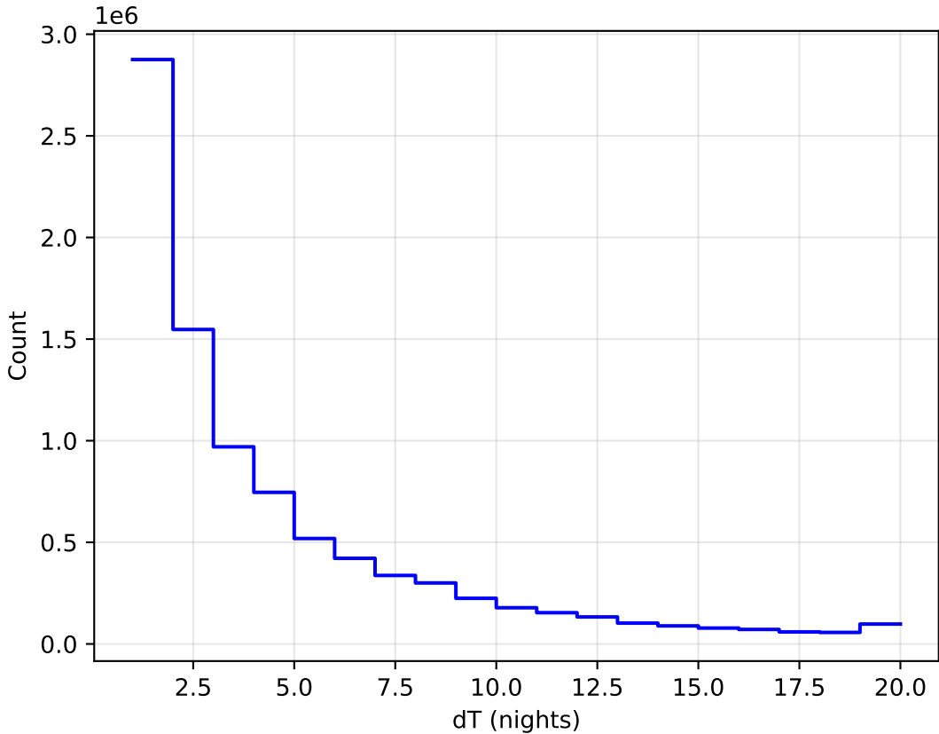
internal_u_expt45_nscale1.2v3.4_10yrs All sky all bands: DeltaNight Histogram
