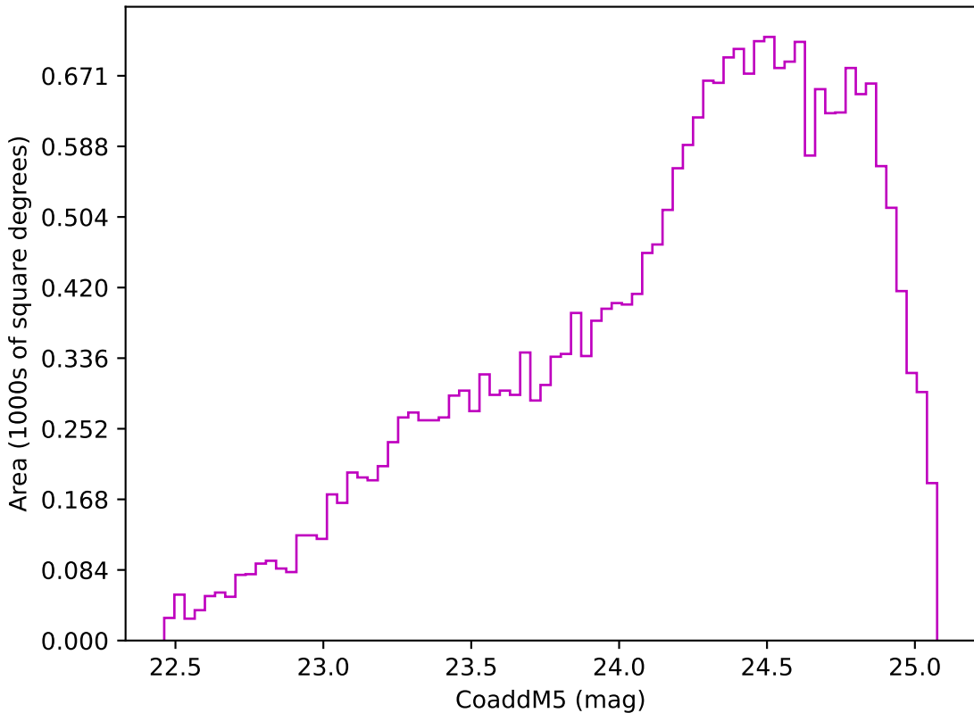
internal_u_expt45_nscale1.2v3.4_10yrs Yr 3-4 z band: CoaddM5
