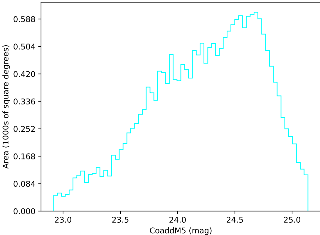
internal_u_expt45_nscale1.2v3.4_10yrs Yr 3-4 u band: CoaddM5
