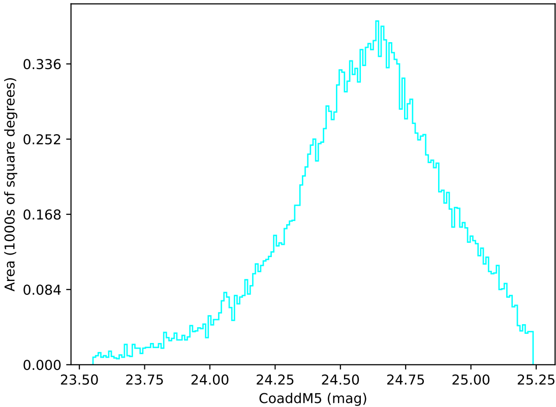
internal_u_expt45_nscale1.2v3.4_10yrs Yr 1 u band: CoaddM5
