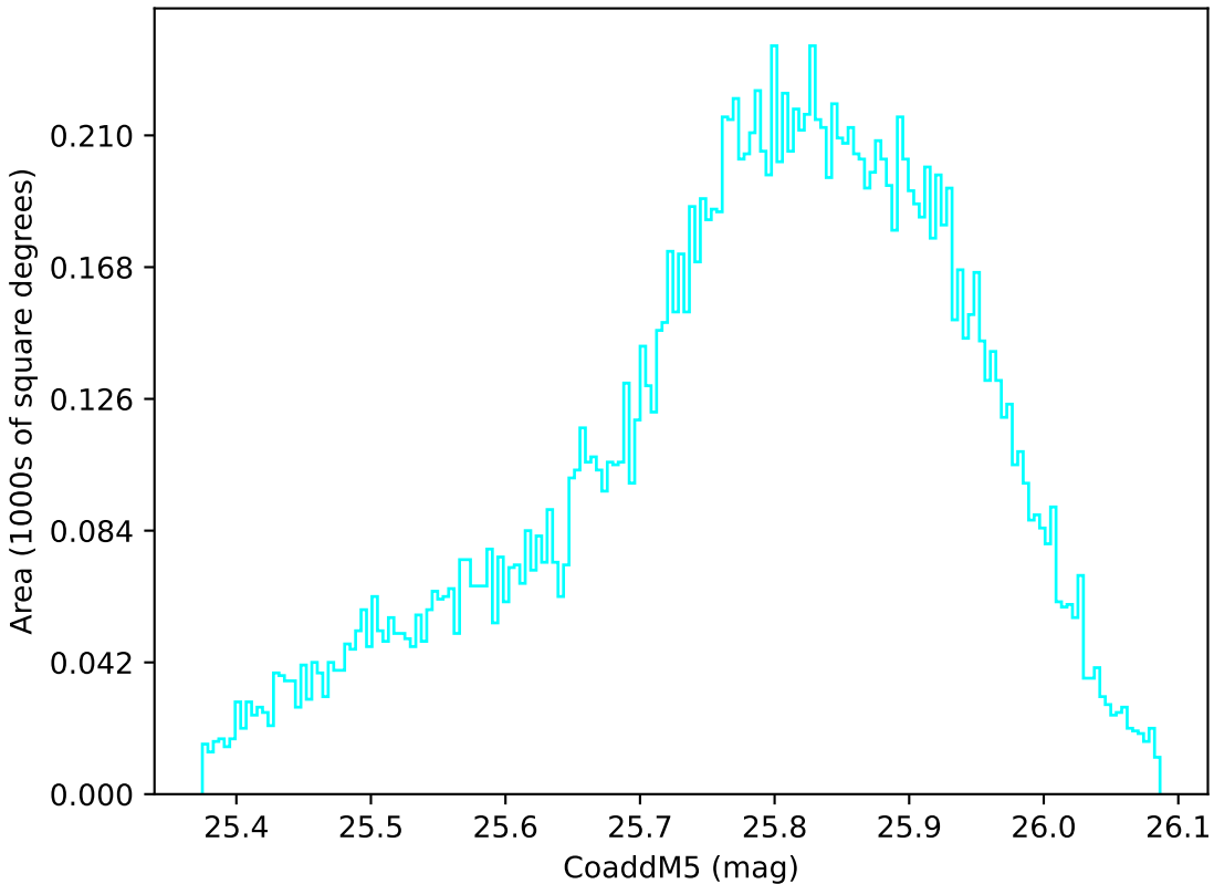
internal_u_expt45_nscale1.2v3.4_10yrs WFD u band: CoaddM5
