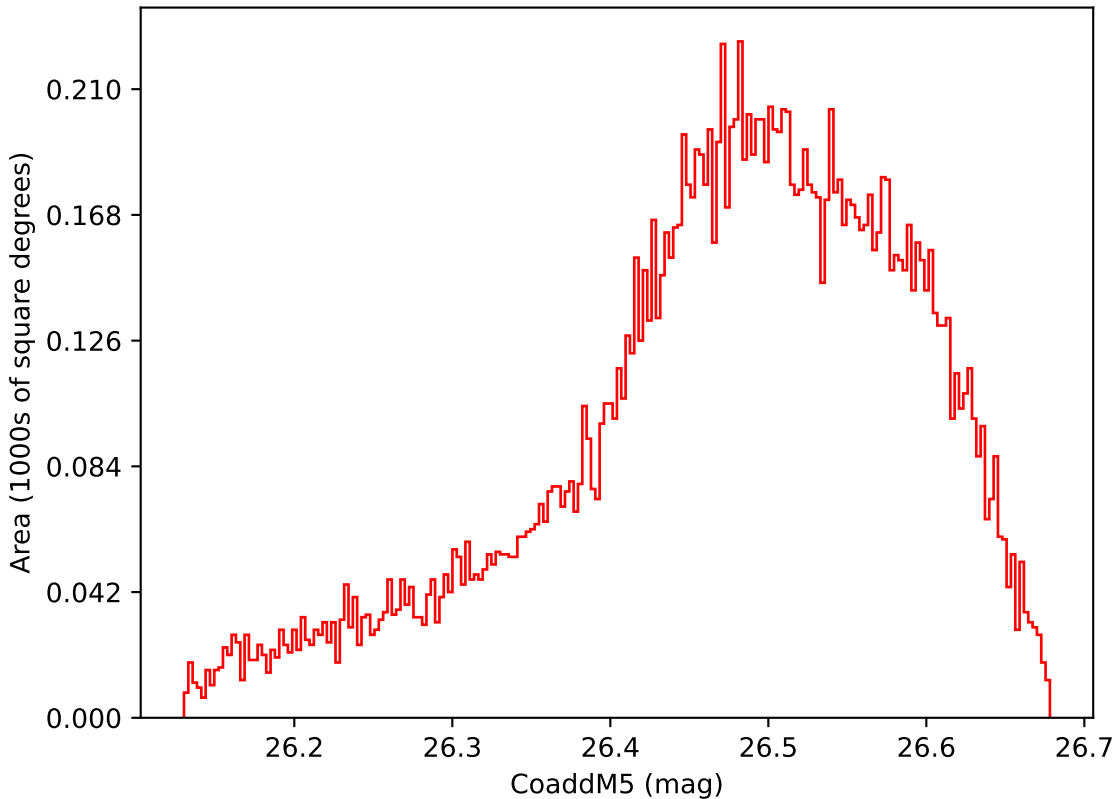
internal_u_expt45_nscale1.2v3.4_10yrs WFD i band: CoaddM5
