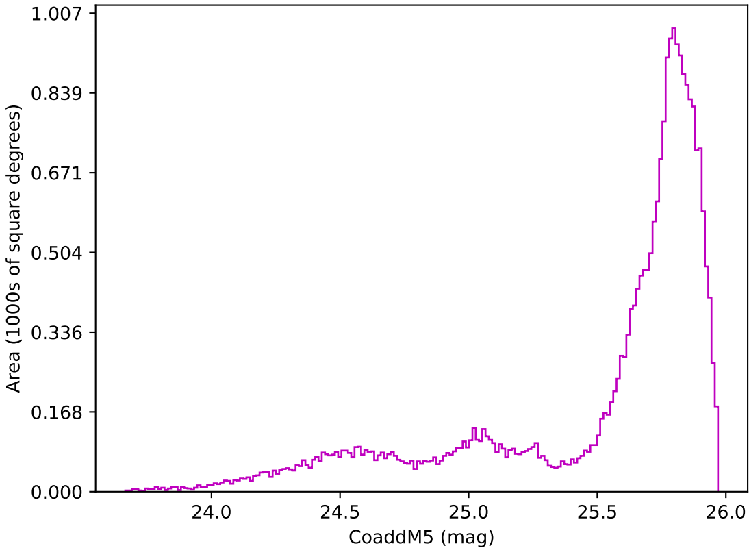
internal_u_expt45_nscale1.2v3.4_10yrs All sky z band: CoaddM5
