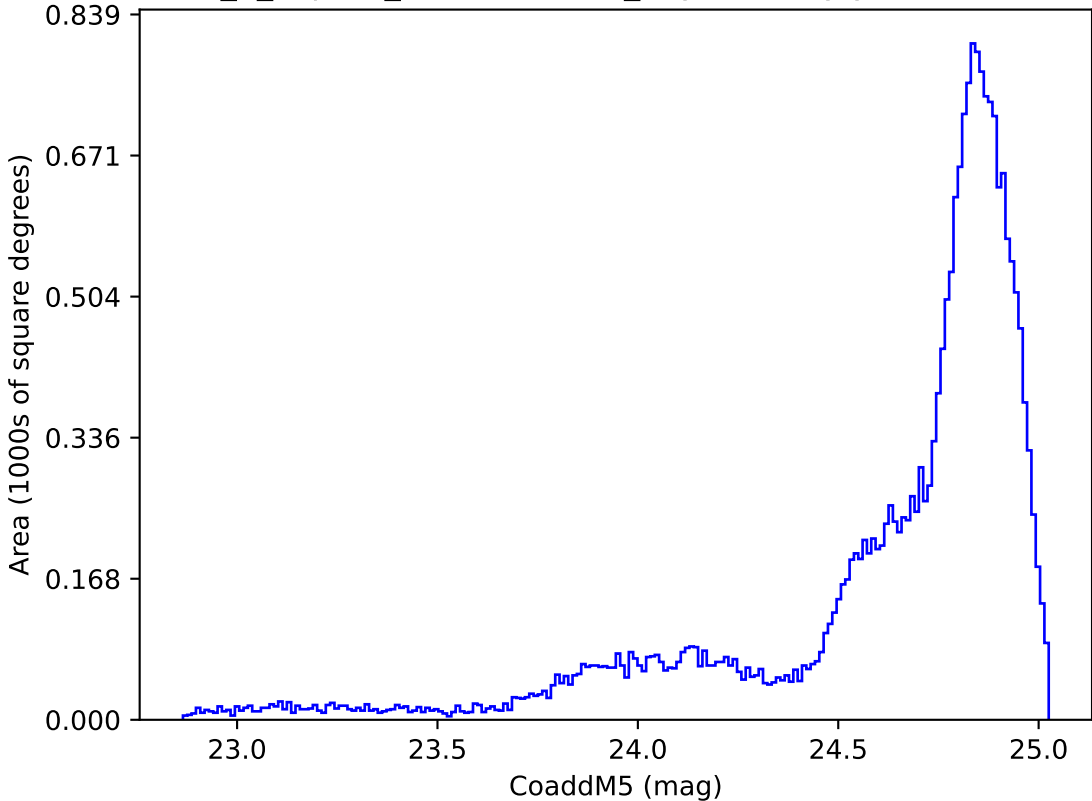
internal_u_expt45_nscale1.2v3.4_10yrs All sky y band: CoaddM5
