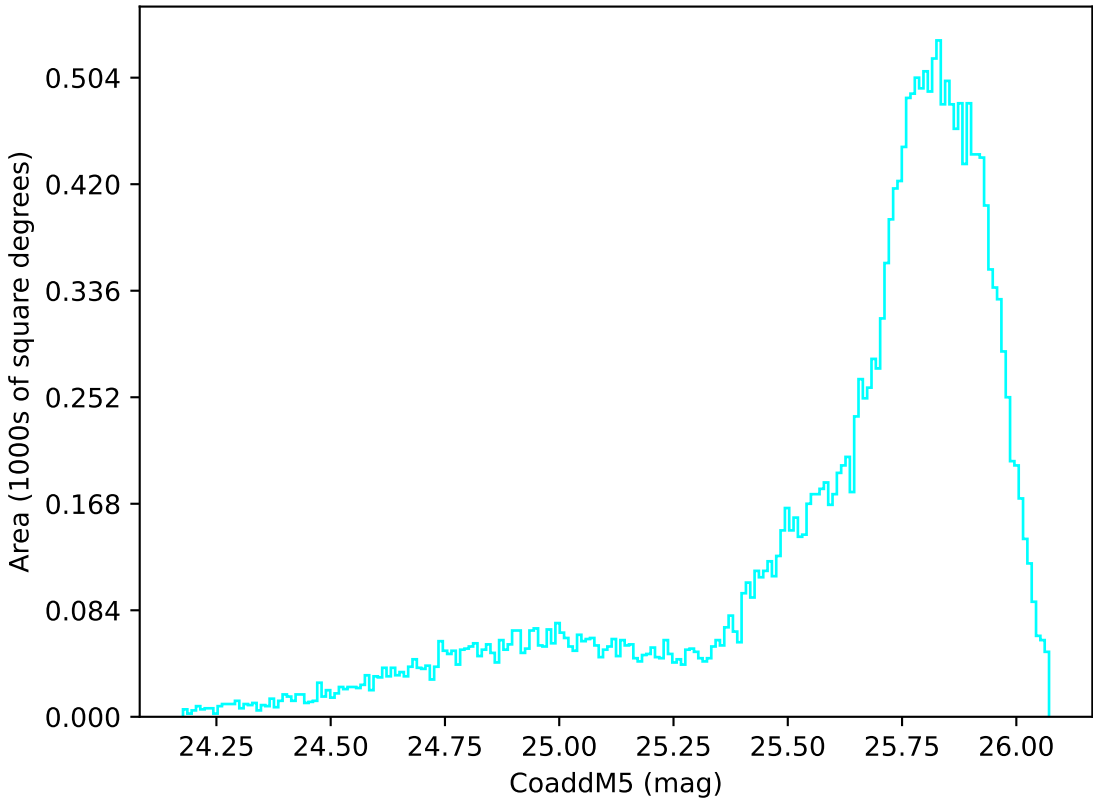
internal_u_expt45_nscale1.2v3.4_10yrs All sky u band: CoaddM5
