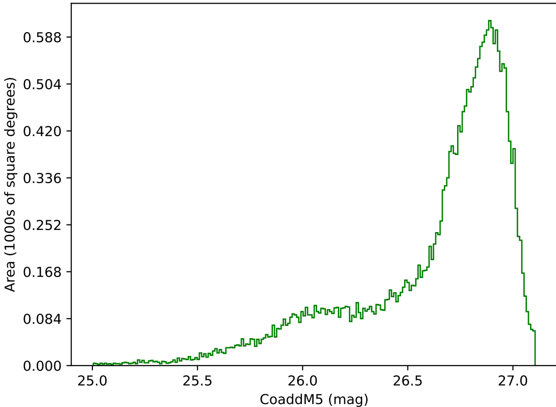
internal_u_expt45_nscale1.2v3.4_10yrs All sky g band: CoaddM5
