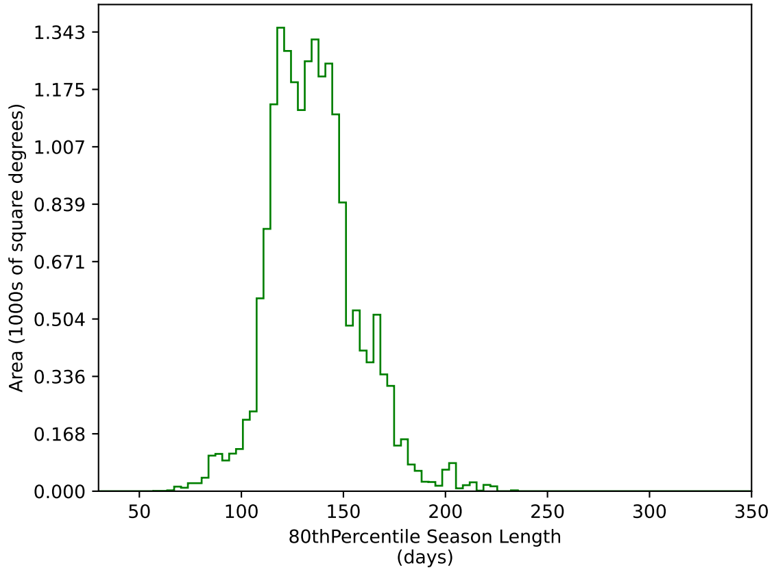
internal_u_expt45_nscale1.2v3.4_10yrs WFD g band: 80thPercentile Season Length
