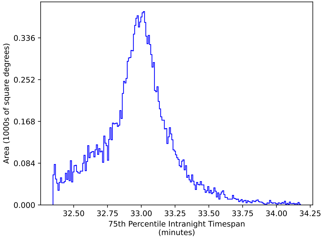
internal_u_expt45_nscale1.2v3.4_10yrs WFD y band: 75th Percentile Intranight Timespan
