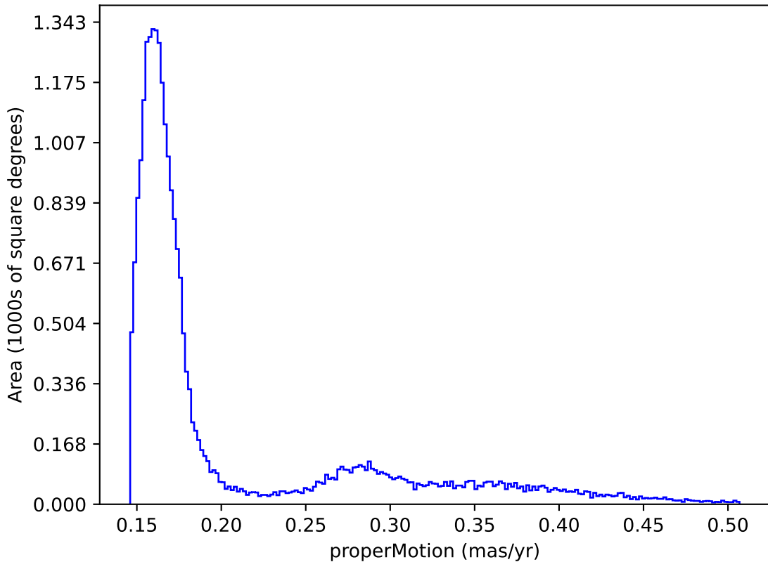
internal_u_expt45_nscale1.2v3.4_10yrs : properMotion
