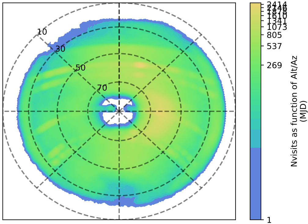
internal_u_expt45_nscale1.2v3.4_10yrs z: Nvisits as function of Alt/Az
