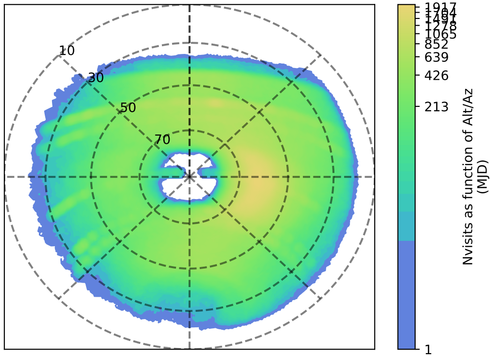
internal_u_expt45_nscale1.2v3.4_10yrs y: Nvisits as function of Alt/Az
