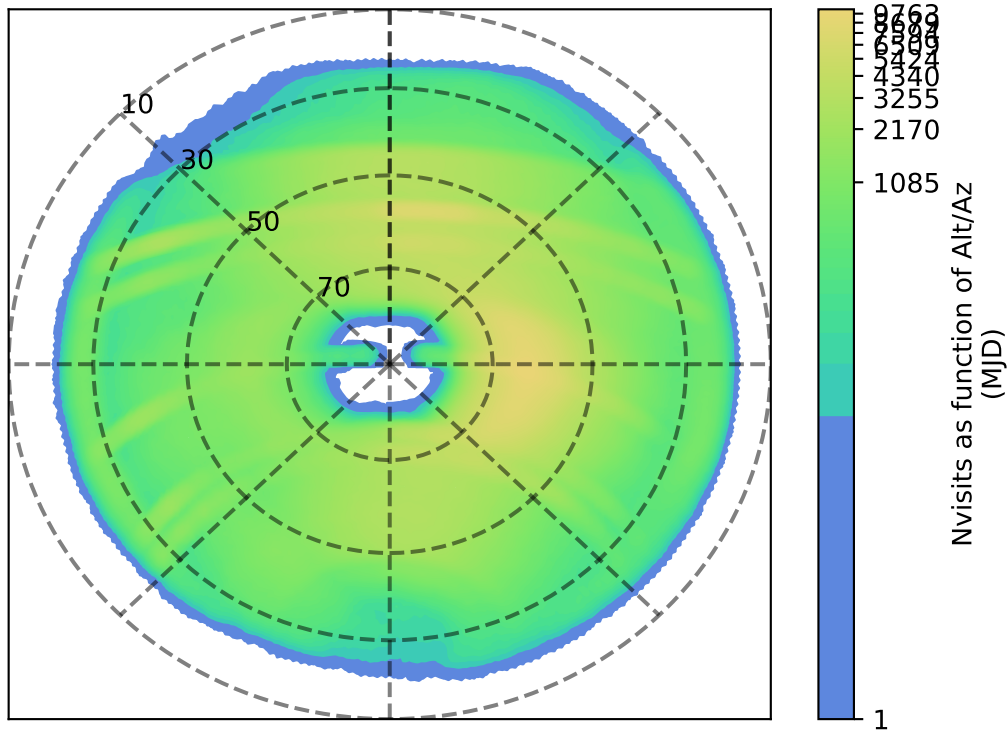
internal_u_expt45_nscale1.2v3.4_10yrs : Nvisits as function of Alt/Az
