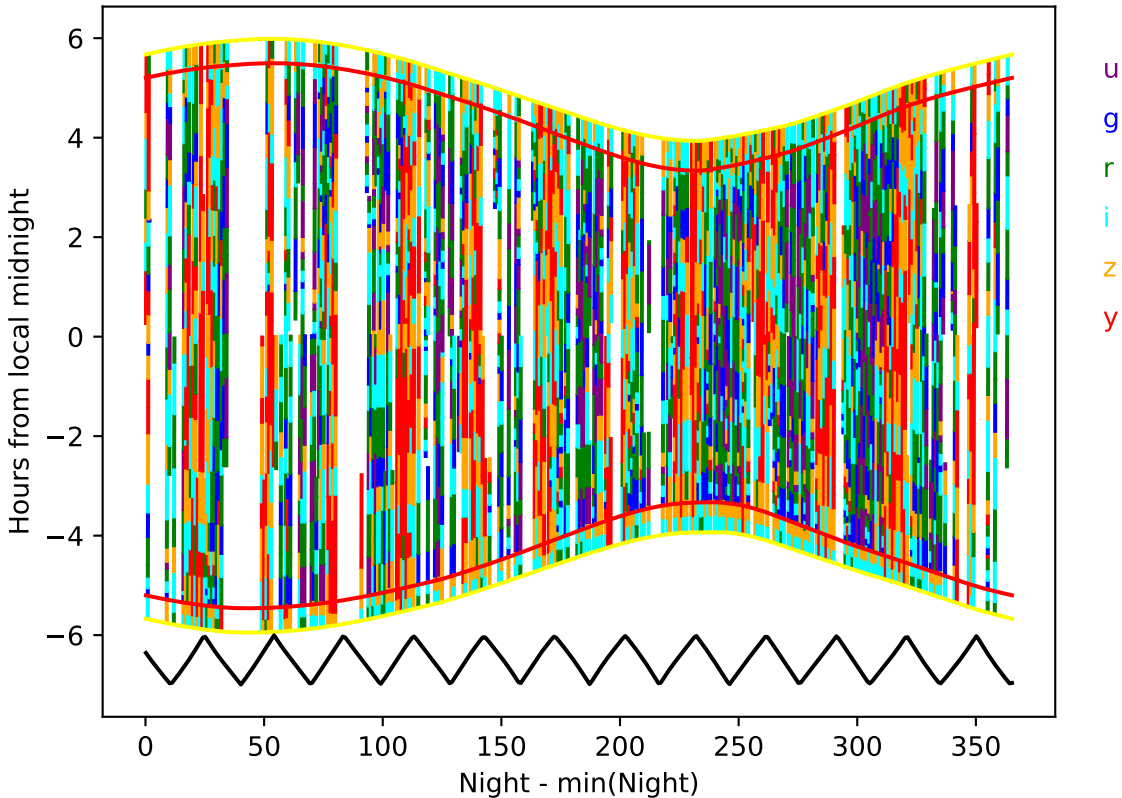
internal_u_expt45_nscale1.2v3.4_10yrs year 4-5: Hourglass
