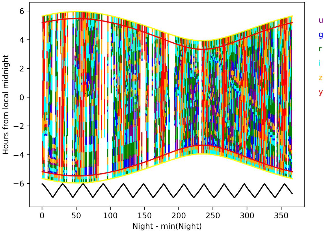
internal_u_expt45_nscale1.2v3.4_10yrs year 1-2: Hourglass
