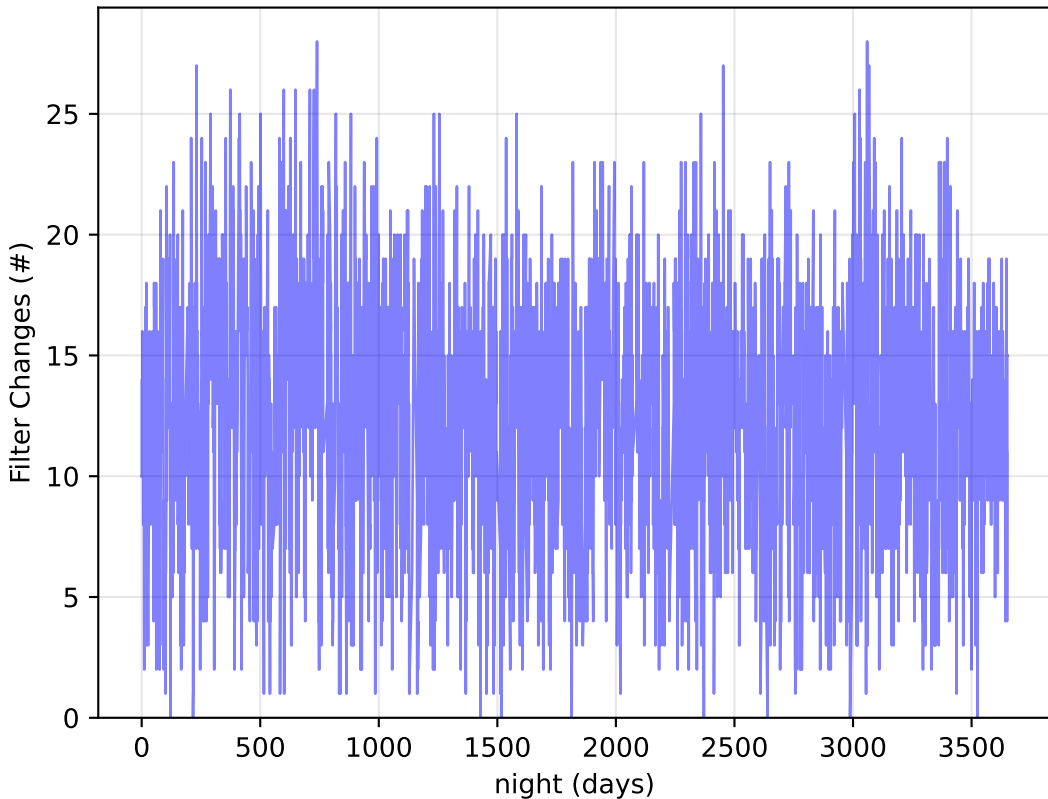
internal_u_expt45_nscale1.2v3.4_10yrs : Filter Changes
