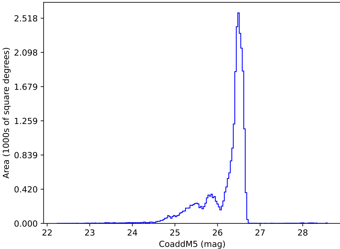
internal_u_expt45_nscale1.2v3.4_10yrs i: CoaddM5
