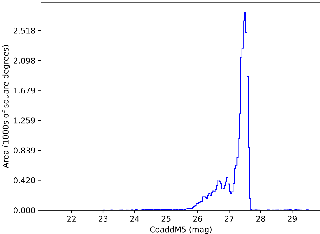
internal_u_expt45_nscale1.2v3.4_10yrs : CoaddM5
