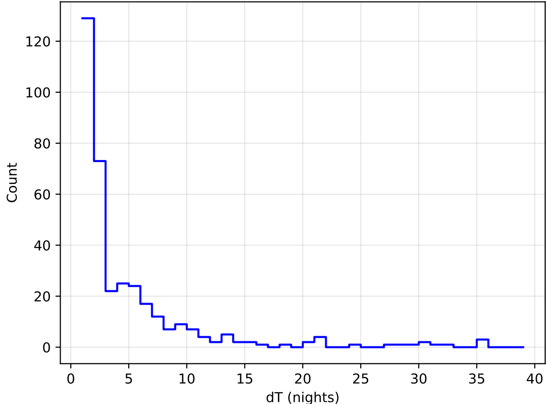
internal_u_expt45_nscale1.2v3.4_10yrs all bands: DD:WFD Delta Nights Histogram
