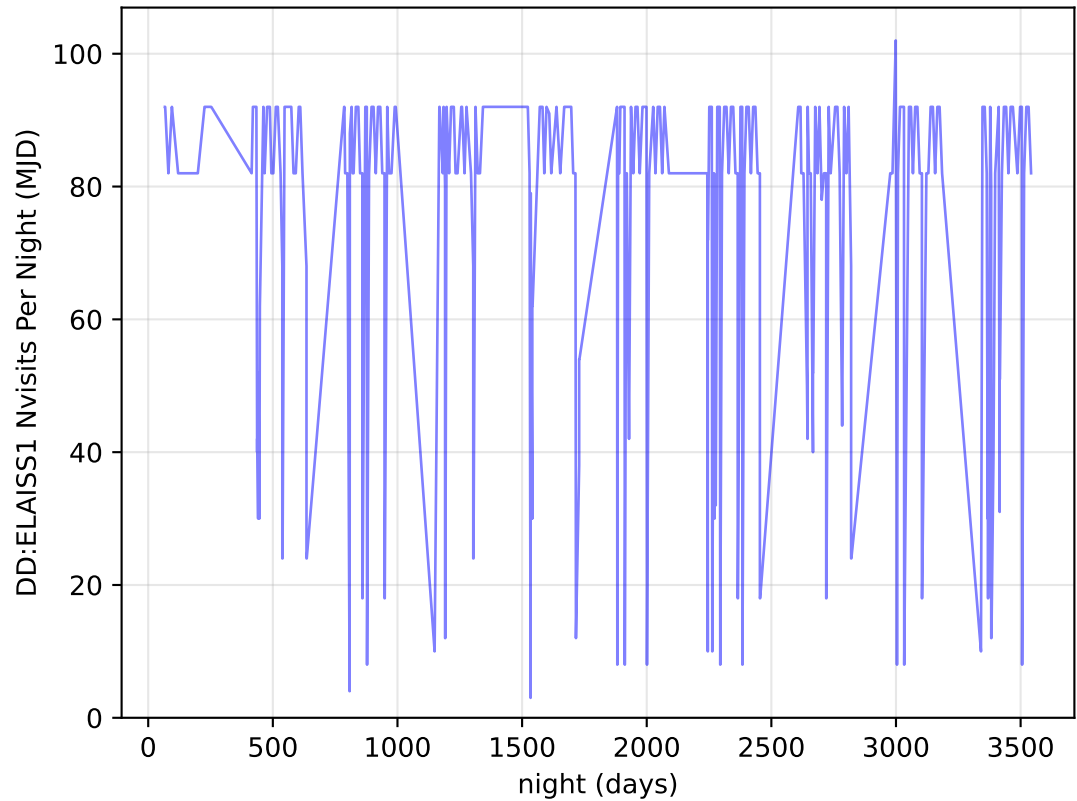
internal_u_expt45_nscale1.2v3.4_10yrs all bands: DD:ELAISS1 Nvisits Per Night
