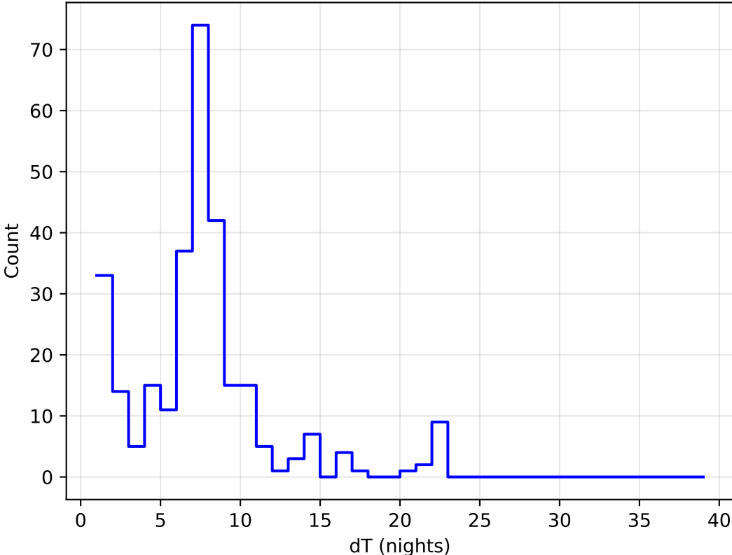
internal_u_expt45_nscale1.2v3.4_10yrs all bands: DD:EDFS Delta Nights Histogram
