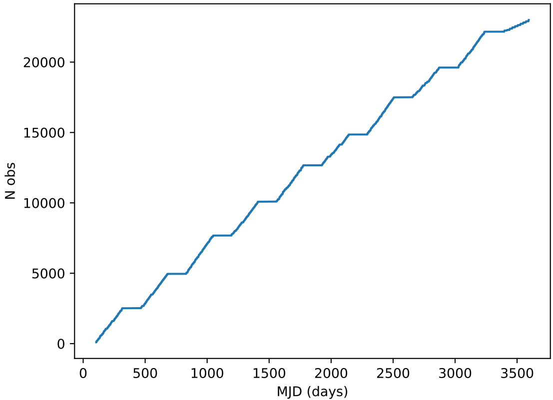
internal_u_expt45_nscale1.2v3.4_10yrs all bands: DD:EDFS Cumulative NVisits
