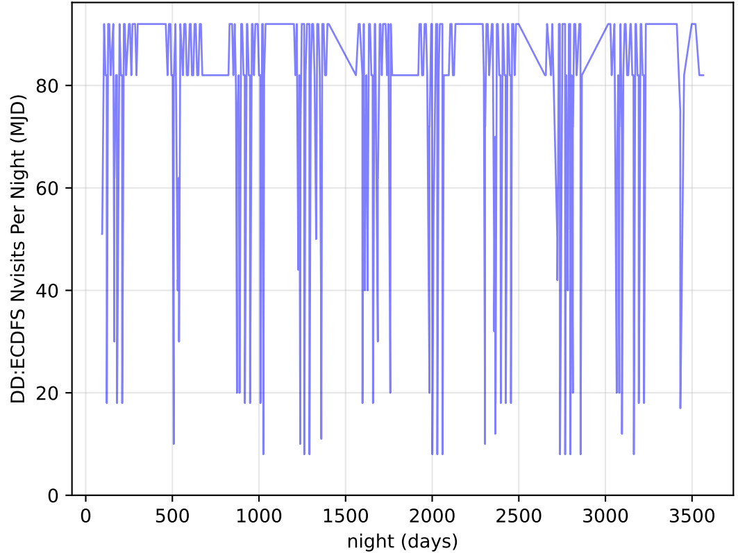
internal_u_expt45_nscale1.2v3.4_10yrs all bands: DD:ECDFS Nvisits Per Night
