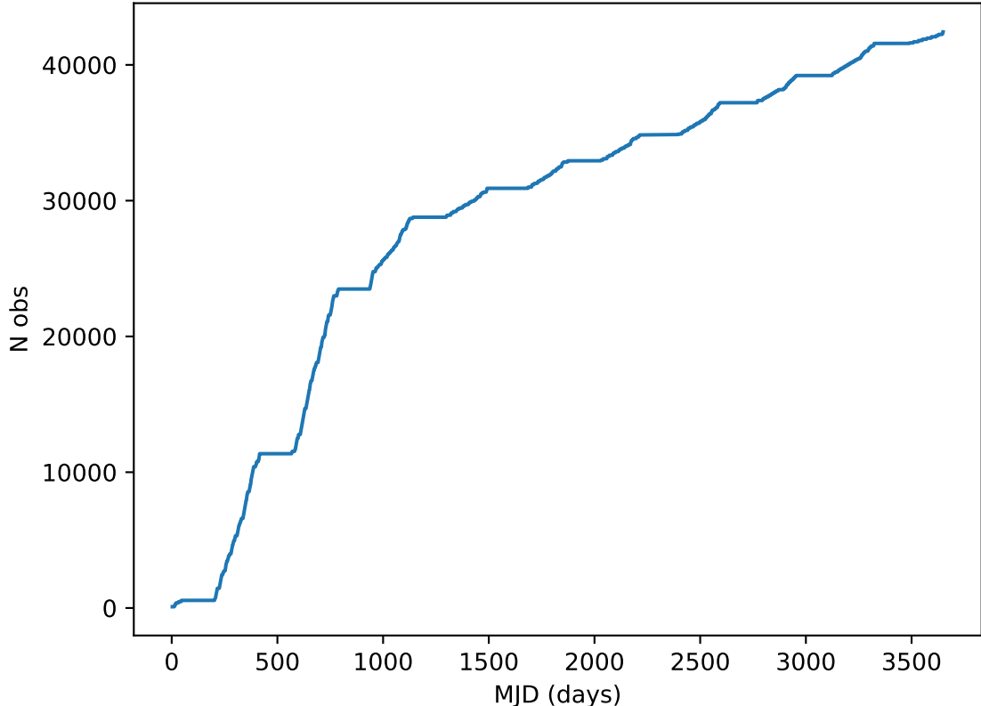
internal_u_expt45_nscale1.2v3.4_10yrs all bands: DD: COSMOS Cumulative NVisits
