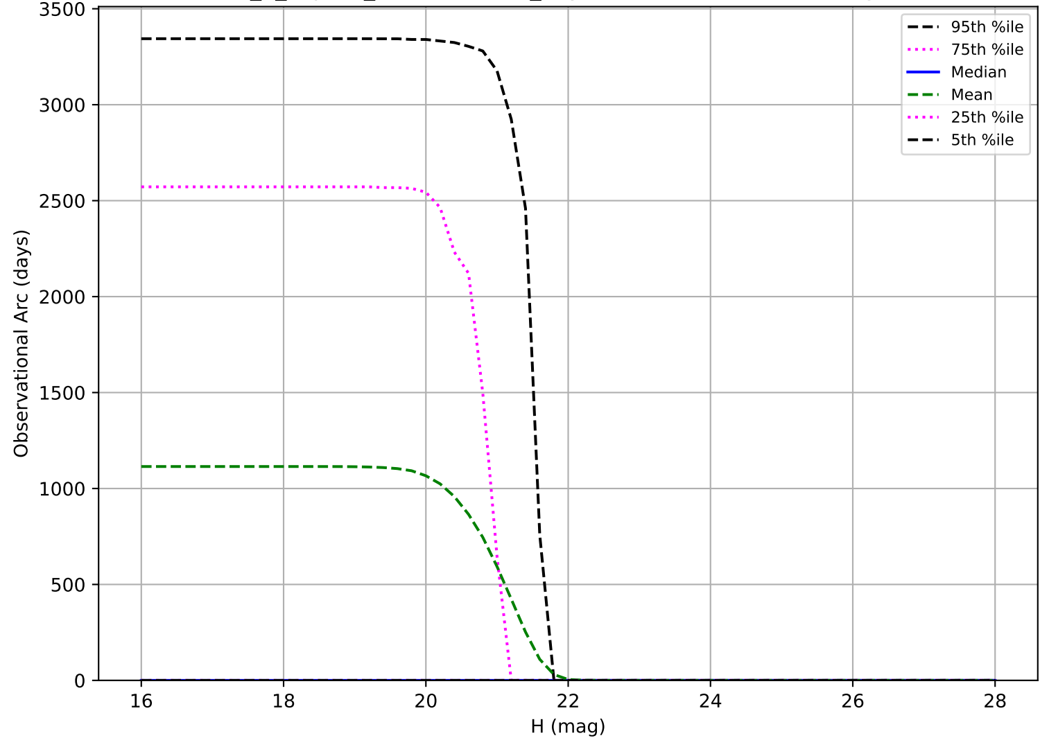
internal_u_expt45_nscale1.1v3.4_10yrs: Observational Arc Length Vatira
