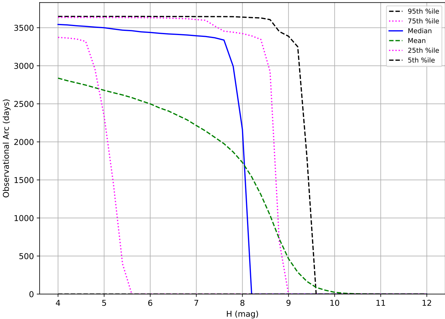
internal_u_expt45_nscale1.1v3.4_10yrs: Observational Arc Length TNO
