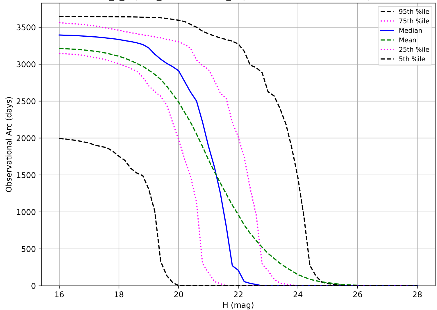
internal_u_expt45_nscale1.1v3.4_10yrs: Observational Arc Length PHA
