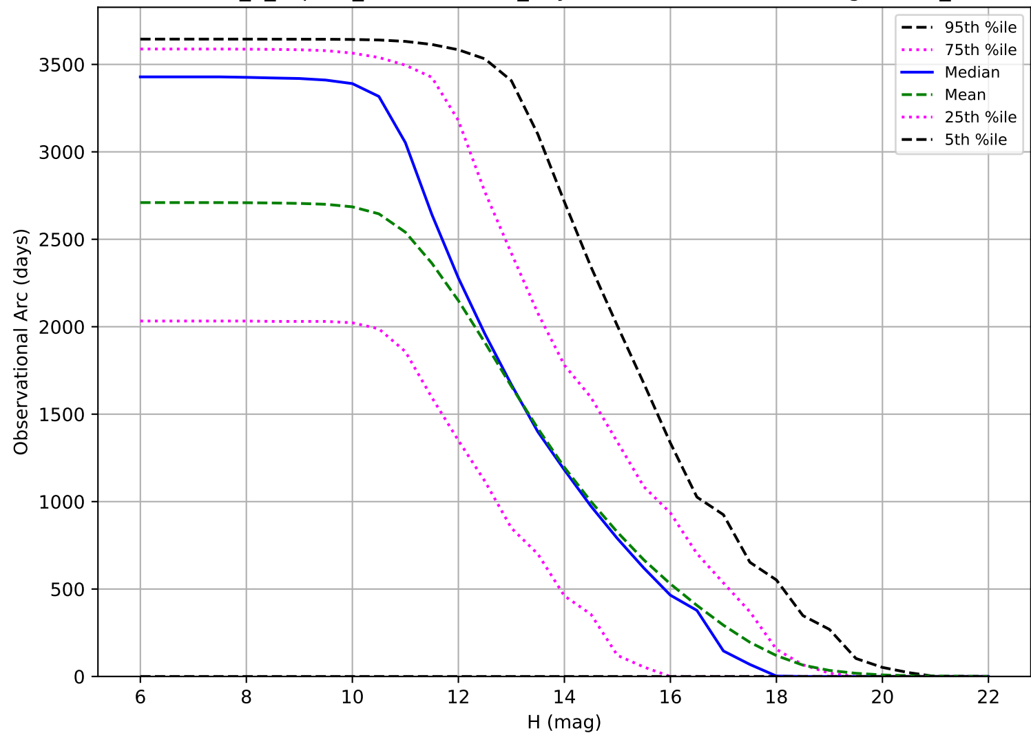
internal_u_expt45_nscale1.1v3.4_10yrs: Observational Arc Length OCC_r5
