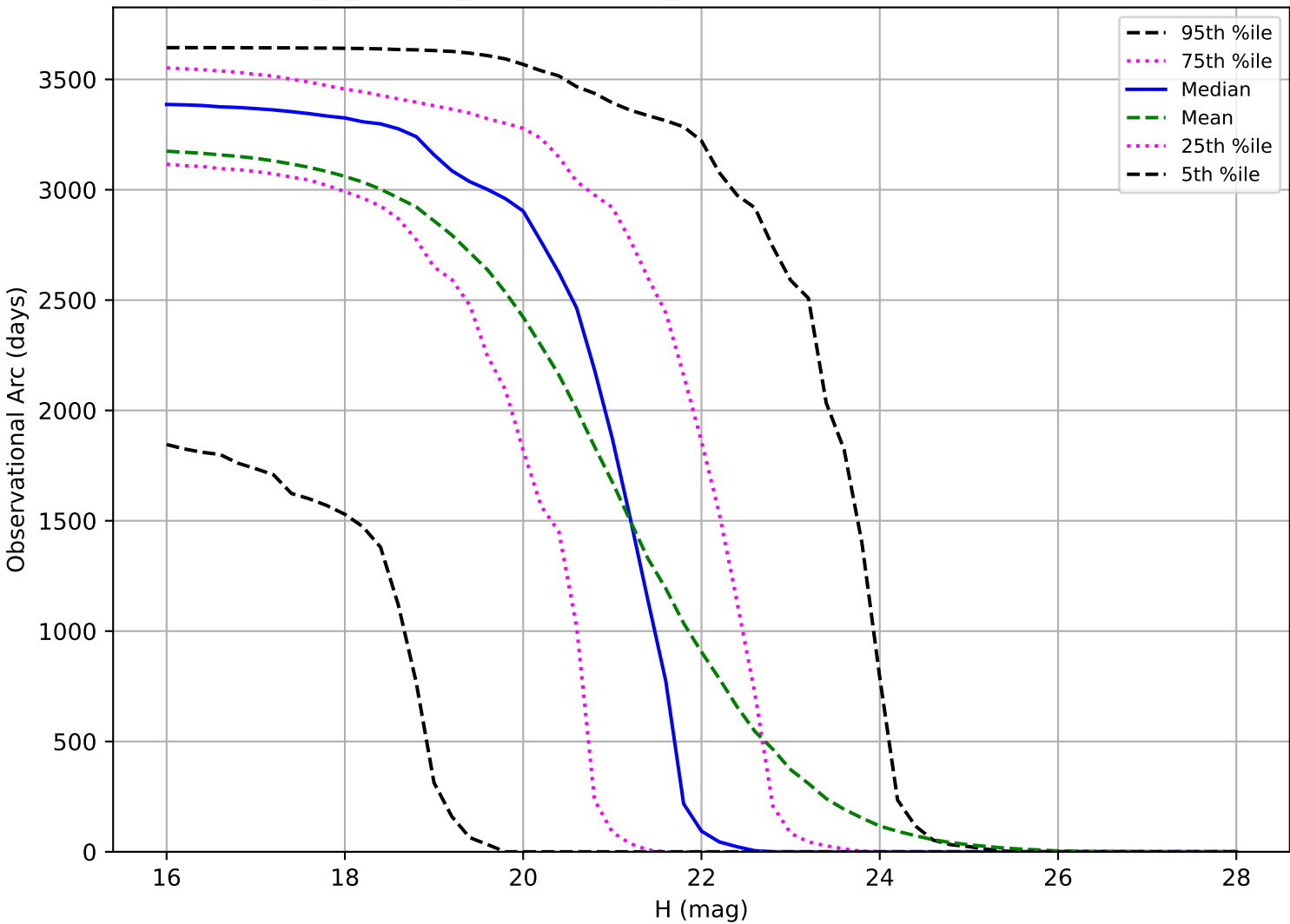
internal_u_expt45_nscale1.1v3.4_10yrs: Observational Arc Length NEO
