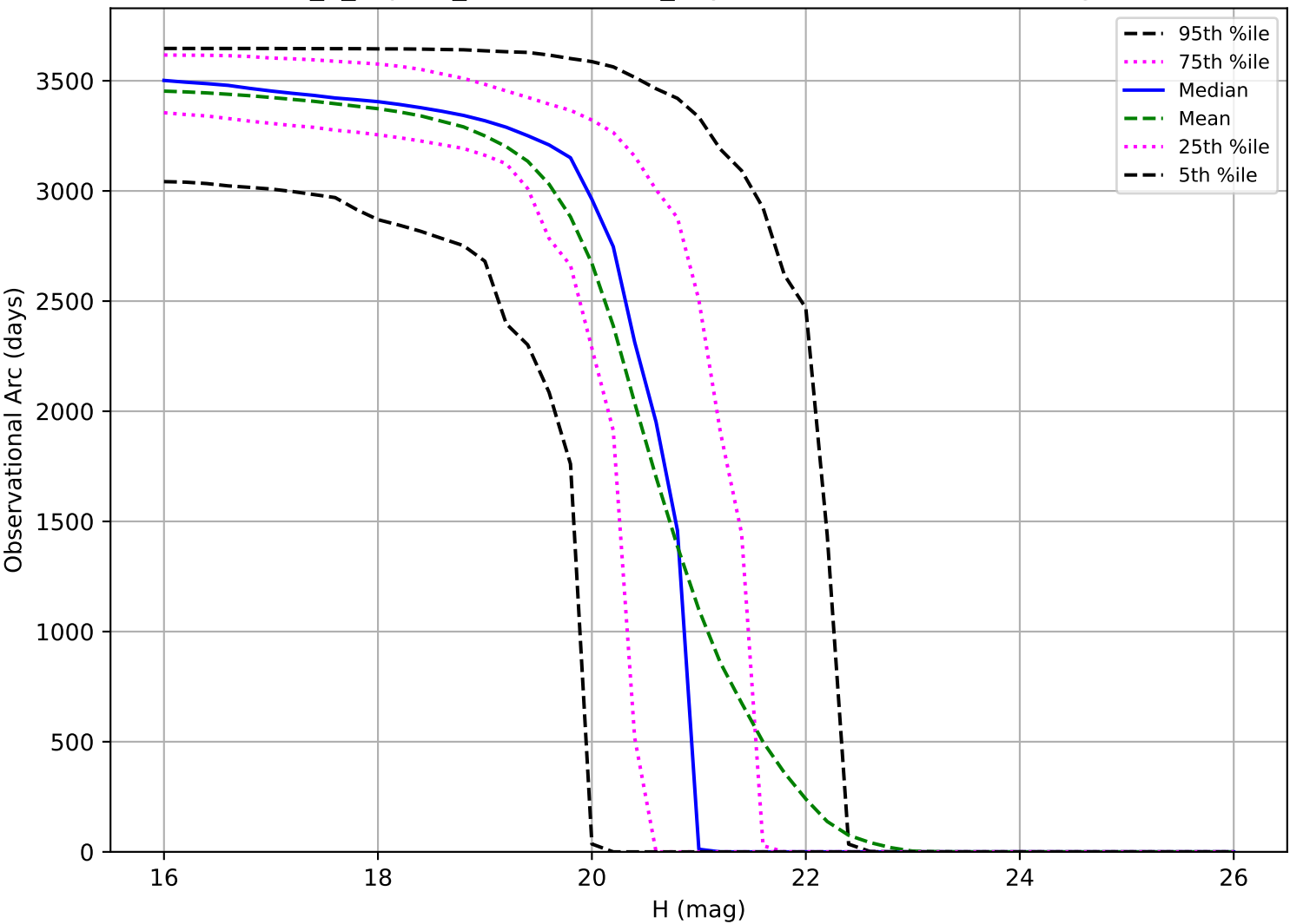
internal_u_expt45_nscale1.1v3.4_10yrs: Observational Arc Length MBA
