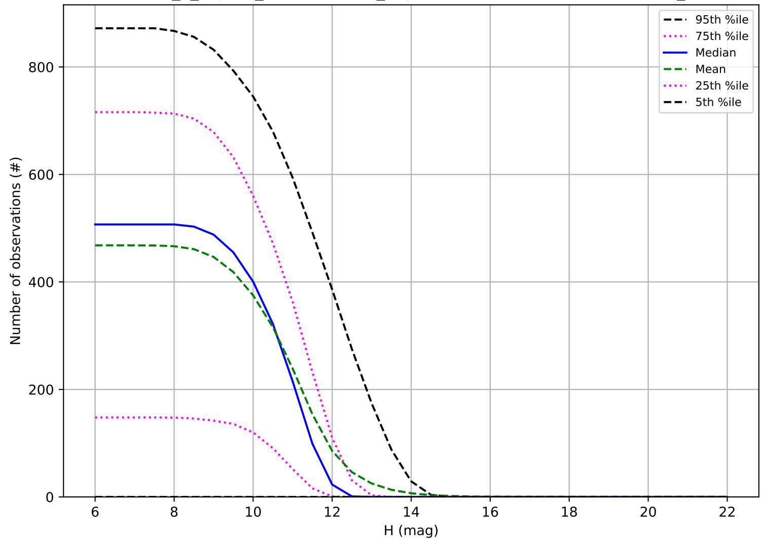
internal_u_expt45_nscale1.1v3.4_10yrs: Number of observations OCC_r20
