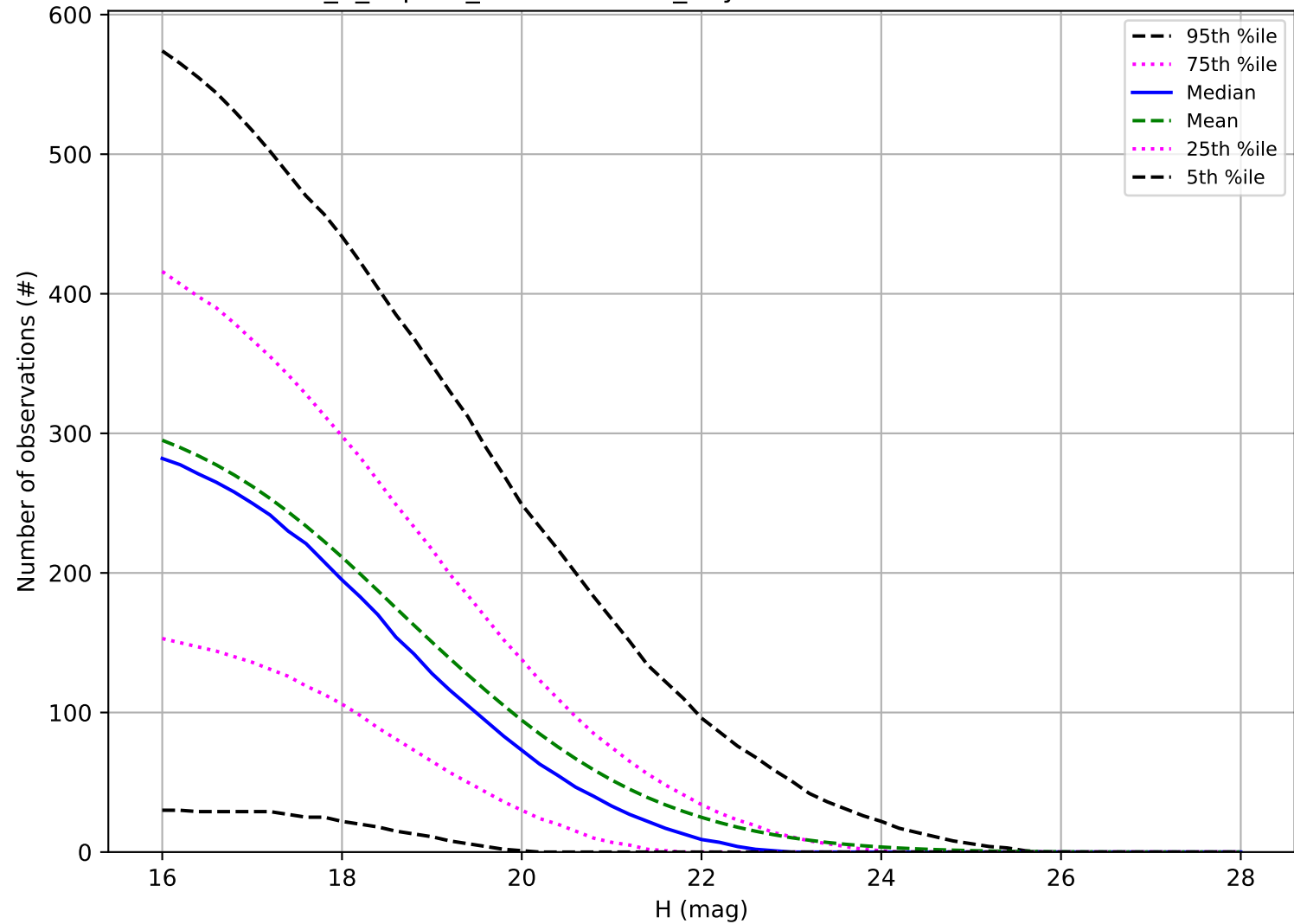
internal_u_expt45_nscale1.1v3.4_10yrs: Number of observations NEO
