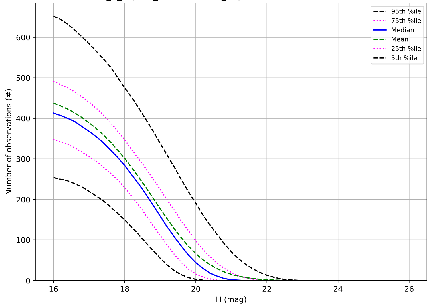
internal_u_expt45_nscale1.1v3.4_10yrs: Number of observations MBA
