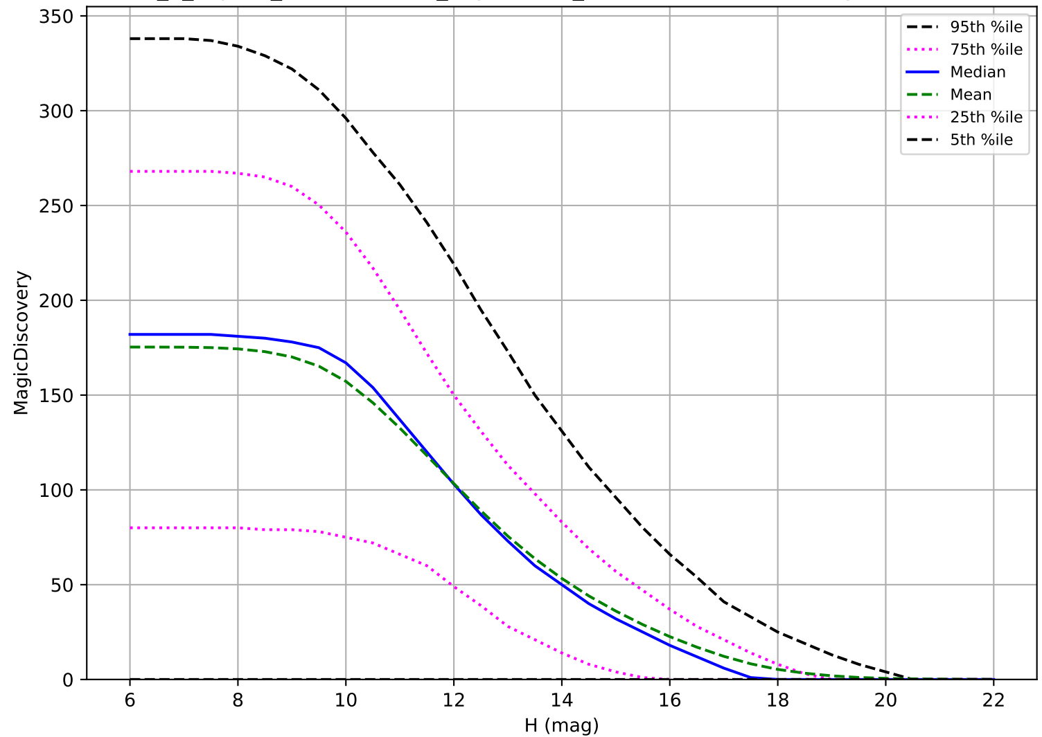
internal_u_expt45_nscale1.1v3.4_10yrs: OCC_r5 6 detections in 60 nights detection loss
