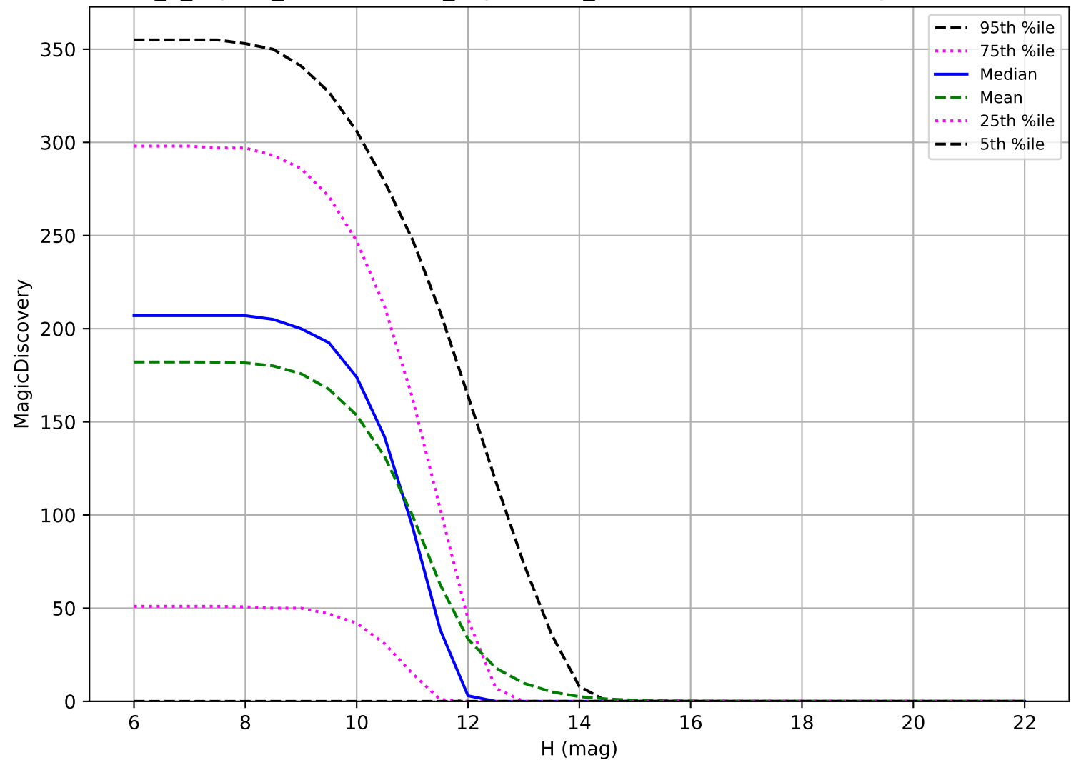
internal_u_expt45_nscale1.1v3.4_10yrs: OCC_r20 6 detections in 60 nights detection loss
