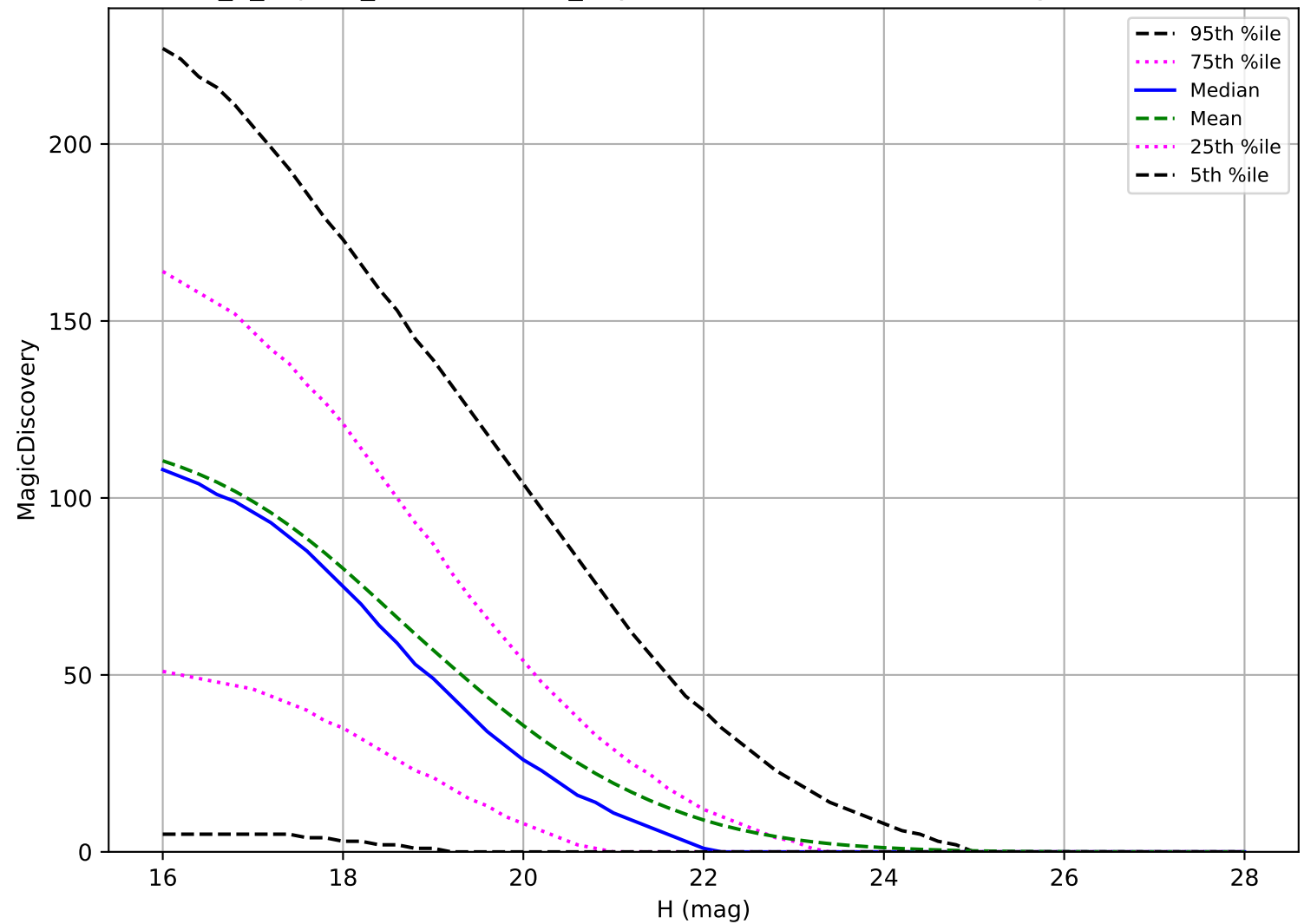
internal_u_expt45_nscale1.1v3.4_10yrs: NEO 6 detections in 60 nights detection loss
