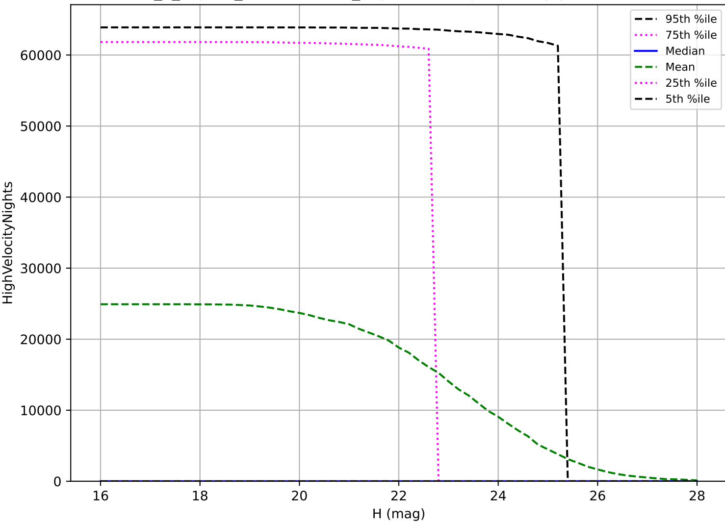
internal_u_expt45_nscale1.1v3.4_10yrs: PHA High velocity pair detection loss
