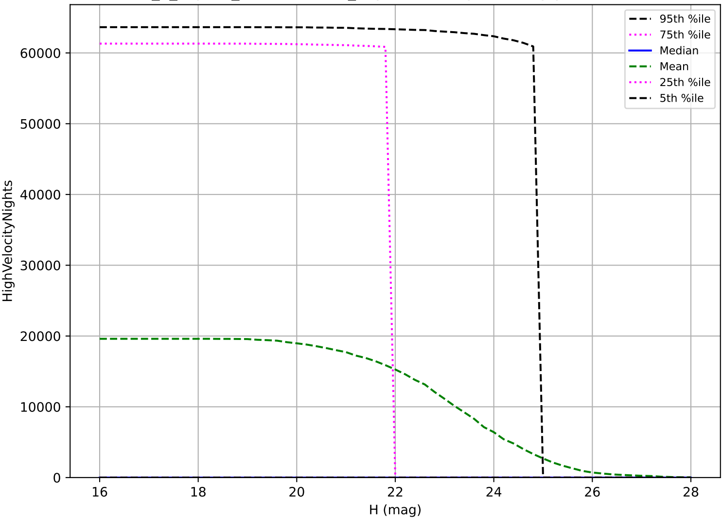
internal_u_expt45_nscale1.1v3.4_10yrs: NEO High velocity pair detection loss
