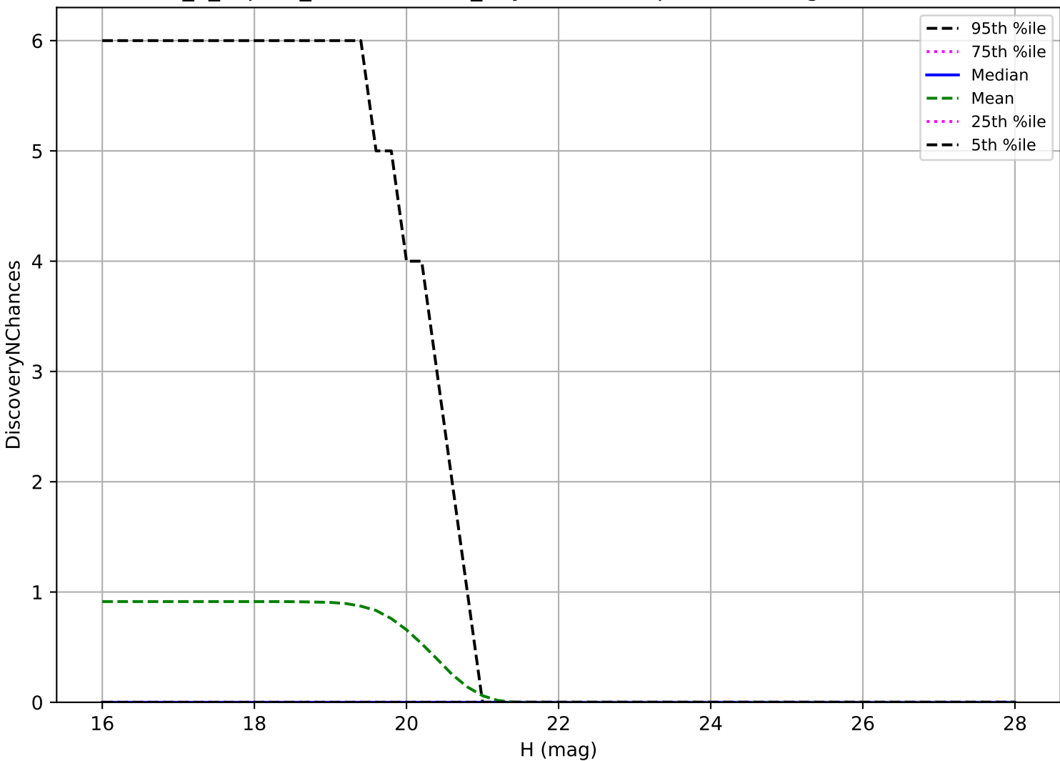
internal_u_expt45_nscale1.1v3.4_10yrs: Vatira 3 pairs in 15 nights detection loss
