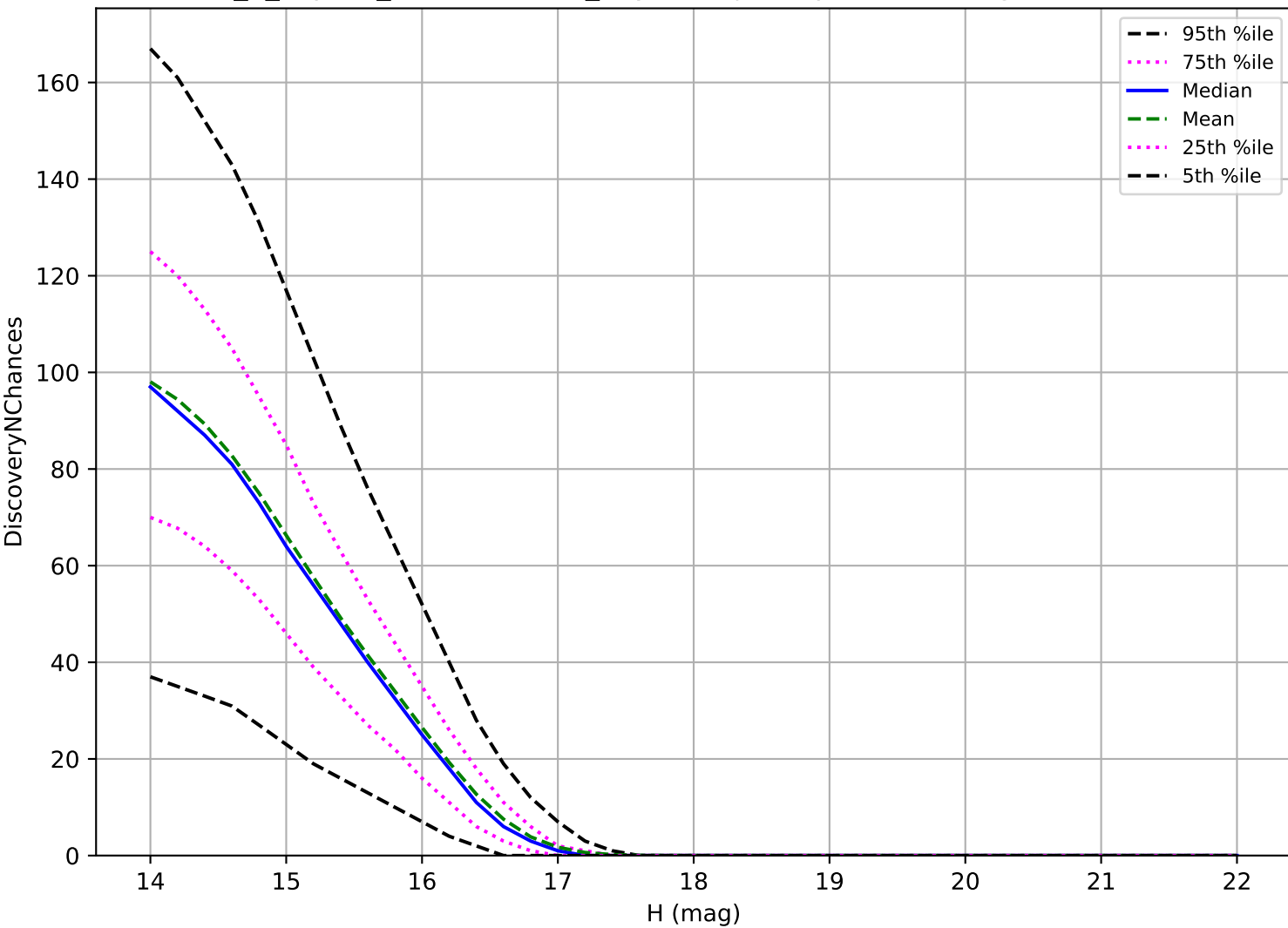
internal_u_expt45_nscale1.1v3.4_10yrs: Trojan 3 pairs in 15 nights detection loss
