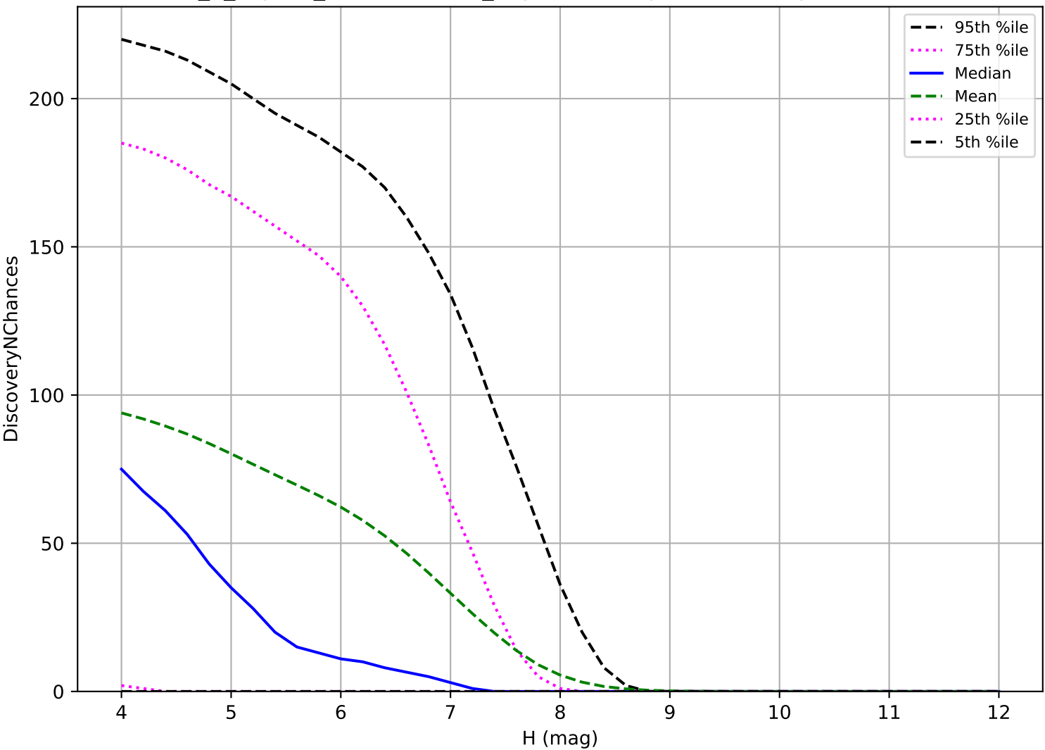
internal_u_expt45_nscale1.1v3.4_10yrs: TNO 3 pairs in 15 nights detection loss
